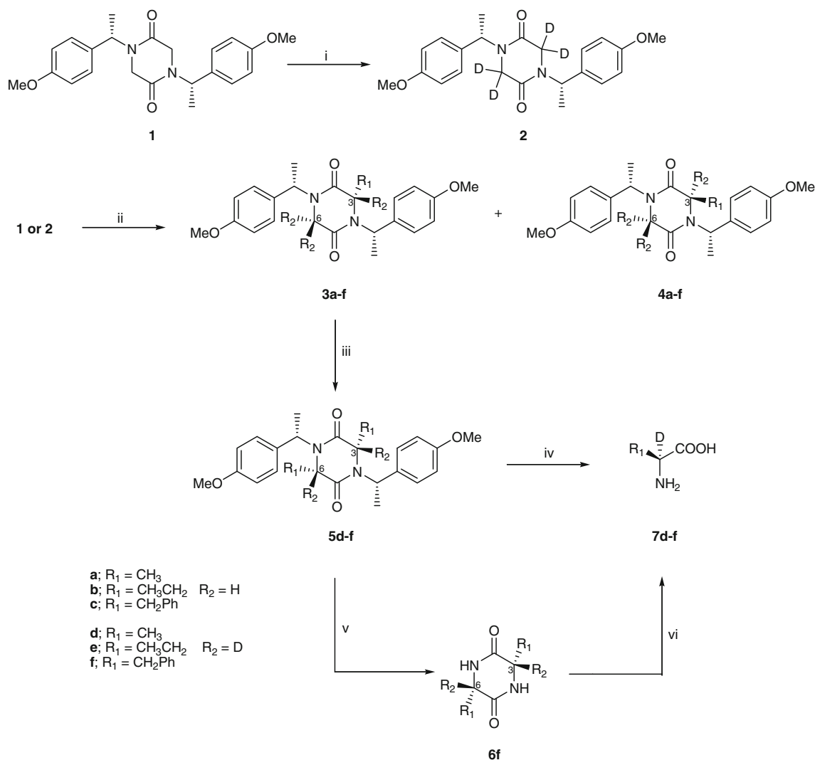
Scheme 1 (i) NaOH, CH_3OD , reflux; (ii) and (iii) LHMDs, anhyd. THF, R-X; (iv) HI, reflux then Dowex resin ( 5d and 5e ) (Balducci et al. 2009b and references therein); (v) CAN, CH_3Cl_2/H_2O (3:2) ( 5f ). (vi) HCl, reflux then Dowex resin
